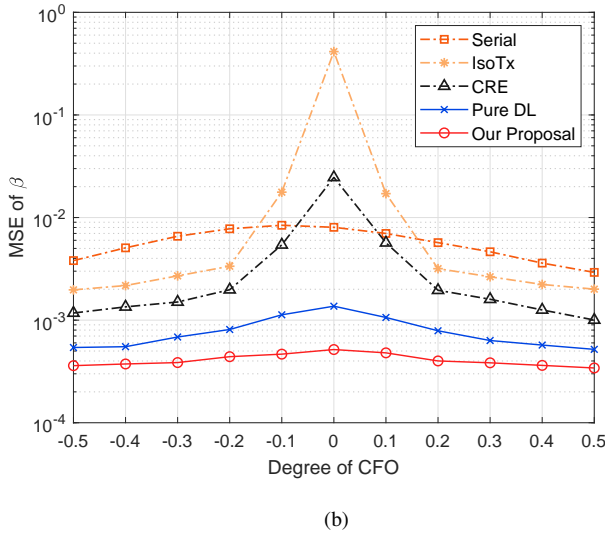
Fig. 6. MSE of IQ imbalance parameters against different CFO degrees: a) MSE of the transmitter IQ imbalance parameter \alpha ; b) MSE of the receiver IQ imbalance parameter \beta .
