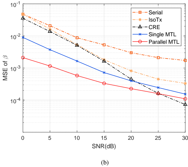
Fig. 4. MSE of IQ imbalance parameters against different SNRs: a) MSE of the transmitter IQ imbalance parameter \alpha ; b) MSE of the receiver IQ imbalance parameter \beta .
