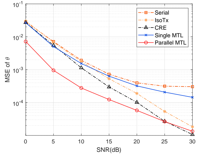
Fig. 3. MSE of CFO parameter \theta against different SNRs.
