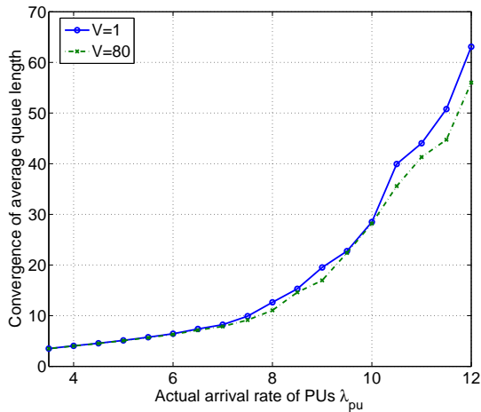
Fig. 4. The convergence of average queue length of PUs as a function of the arrival rate with tradeoff factor V = 1 and V = 80 .
