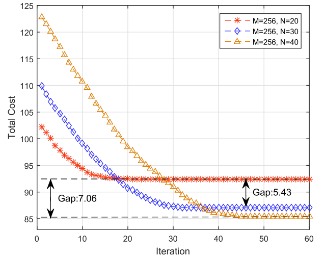
Fig. 2. Total cost during each iteration, \gamma = 0.5 , L = 14km .
