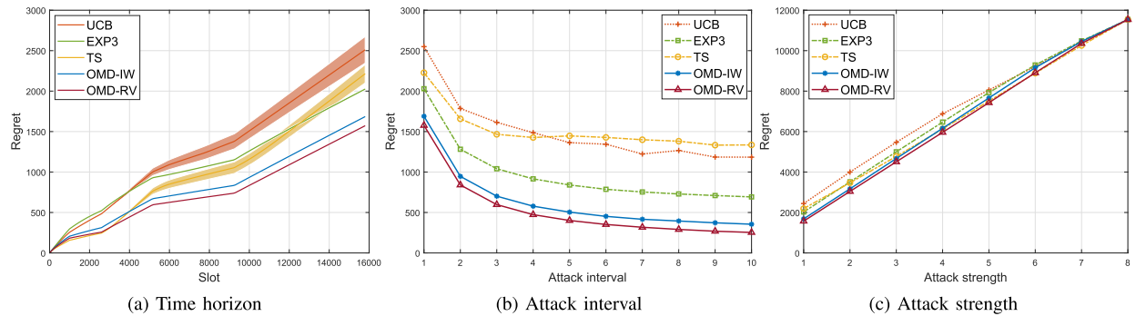
Fig. 4. Regrets in the stochastic regime with adversarial corruptions for the single-SU case with three different system parameters: time horizon T , attack interval \tau and attack strength \xi .
