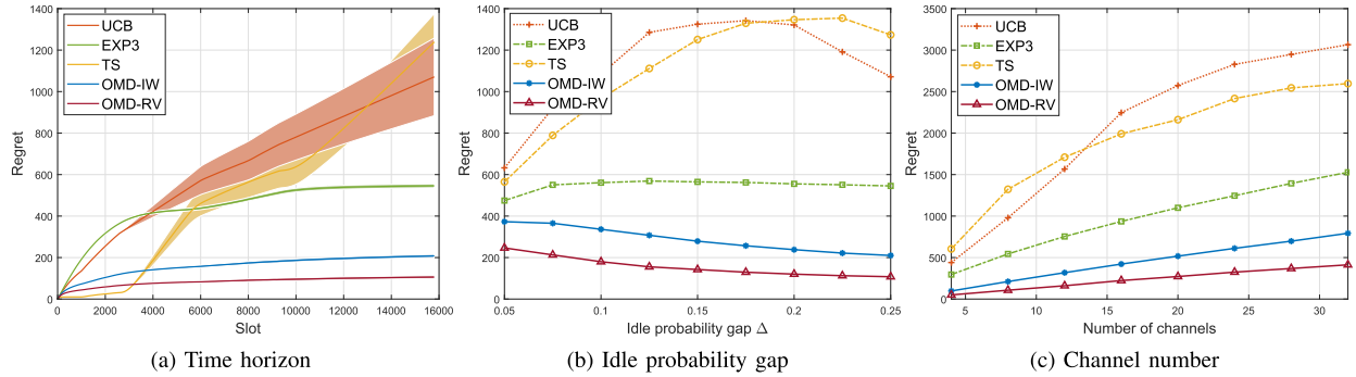
Fig. 3. Regrets in the periodically stochastic regime for the single-SU case with three different system parameters: time horizon T , idle probability gap \Delta and number of channels K .
